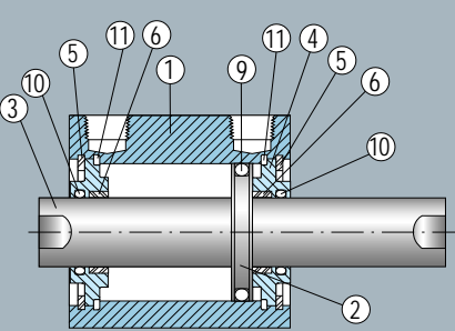
Double Rod/Double Acting
